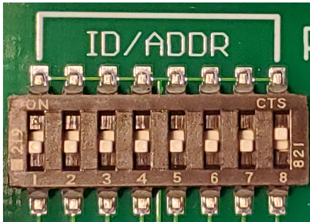
DIP switches - these are all off, so ID 00
