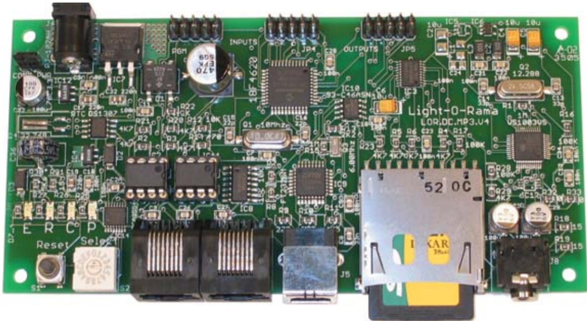
DC-MP3 Board
