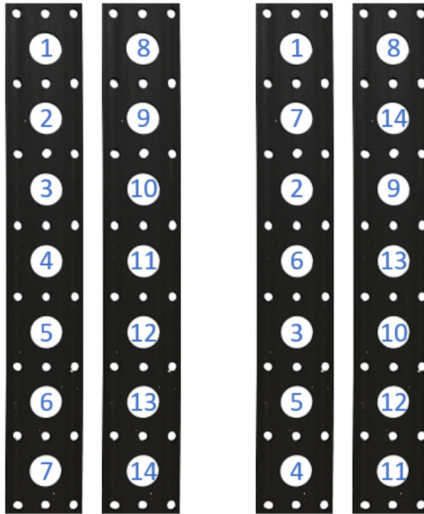
Straight Wiring
