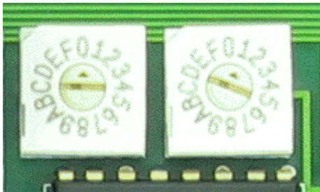
Rotary switches: this pair is set to Unit ID 01
