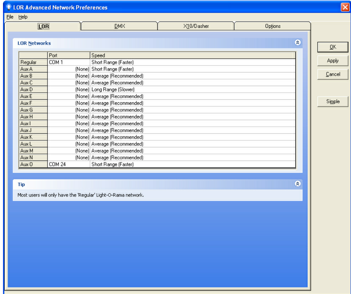
Multiple COM ports assigned to various Light-O-Rama networks
