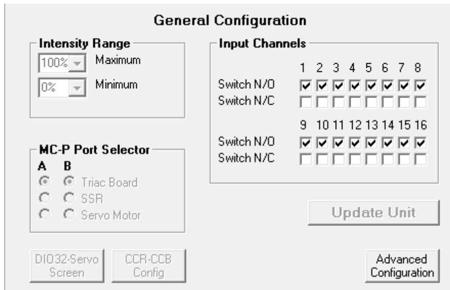
The configuration section of the LOR Control tab
