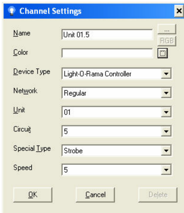
The Visualizer's Channel Settings dialog
